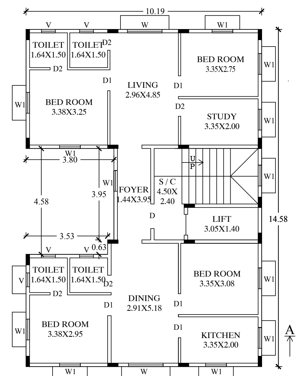
PROPOSED TYPICAL GROUND, FIRST & SECOND FLOOR PLAN
